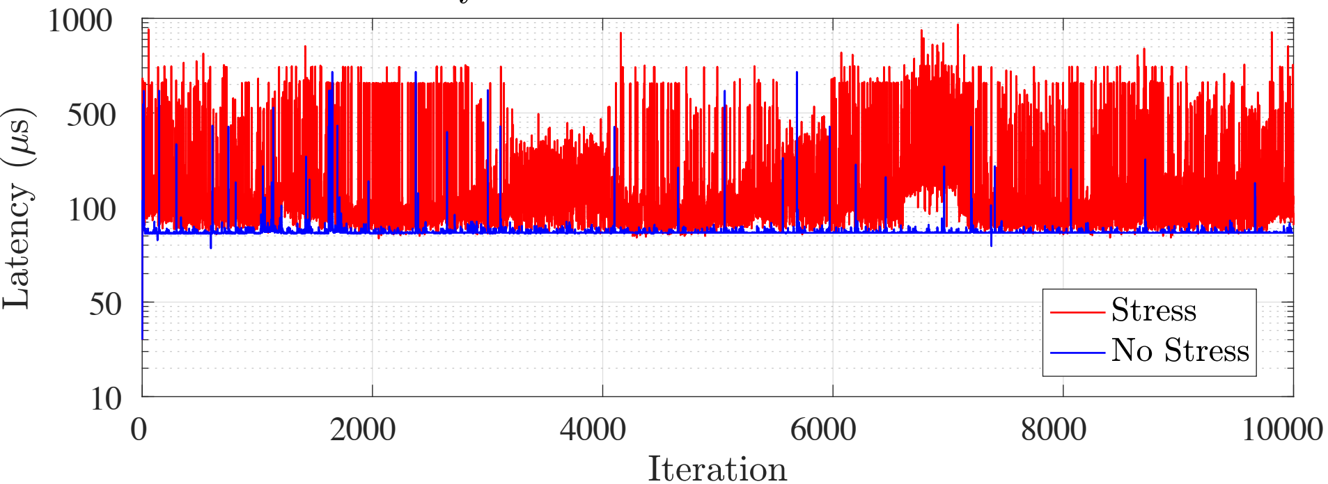
Latency for Scheduler: SCHED_OTHER nice -19
